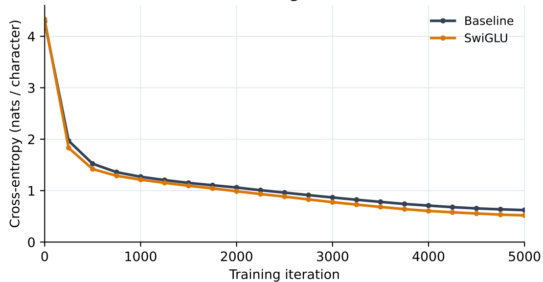
MLP: GELU vs. SwiGLU Training loss
