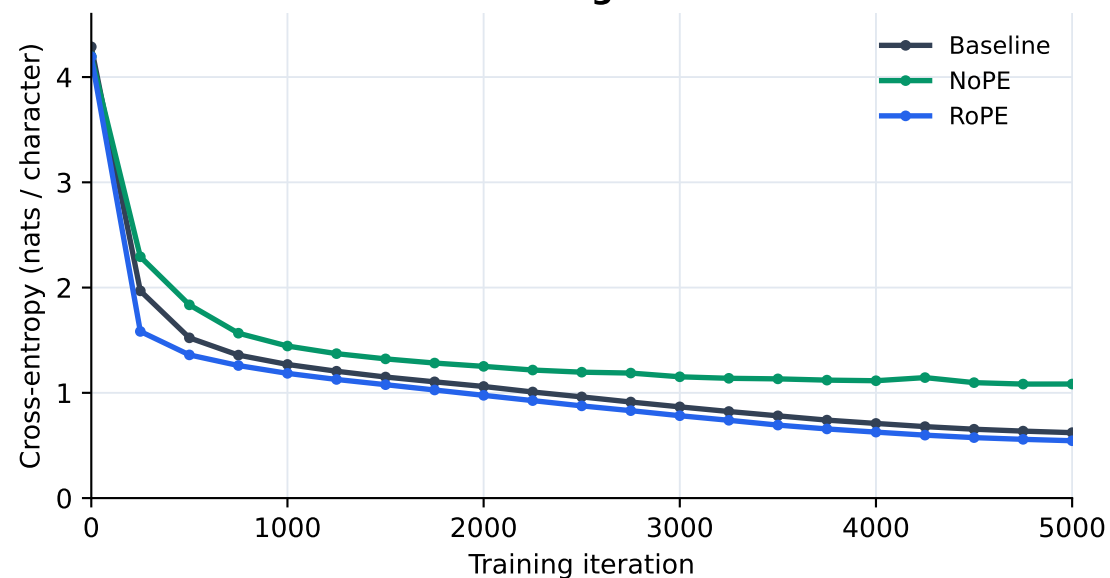
Positions: learned vs. NoPE vs. RoPE Training loss
