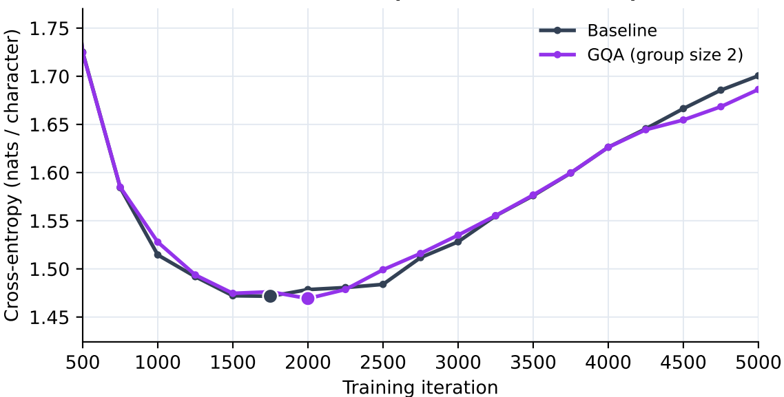
Validation loss (from iteration 500)
