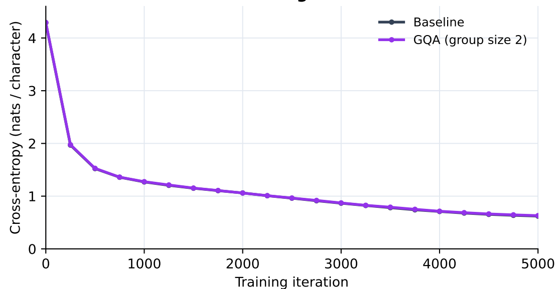
Attention: MHA vs. GQA Training loss
